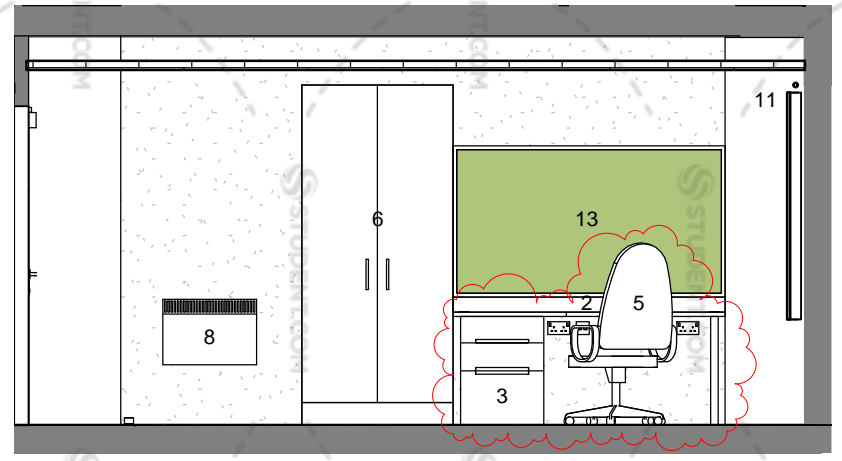
PB1 Elevation 1 1 : 50
