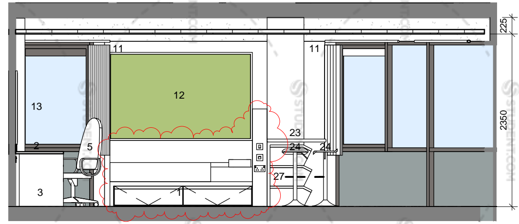
PB1 Elevation 2 1 : 50
