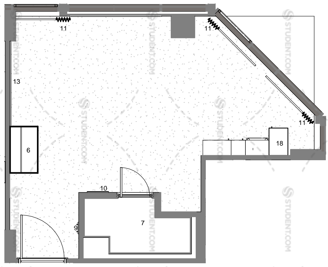
Premium Bedroom 1 Reflected Ceiling Plan 1 : 50
